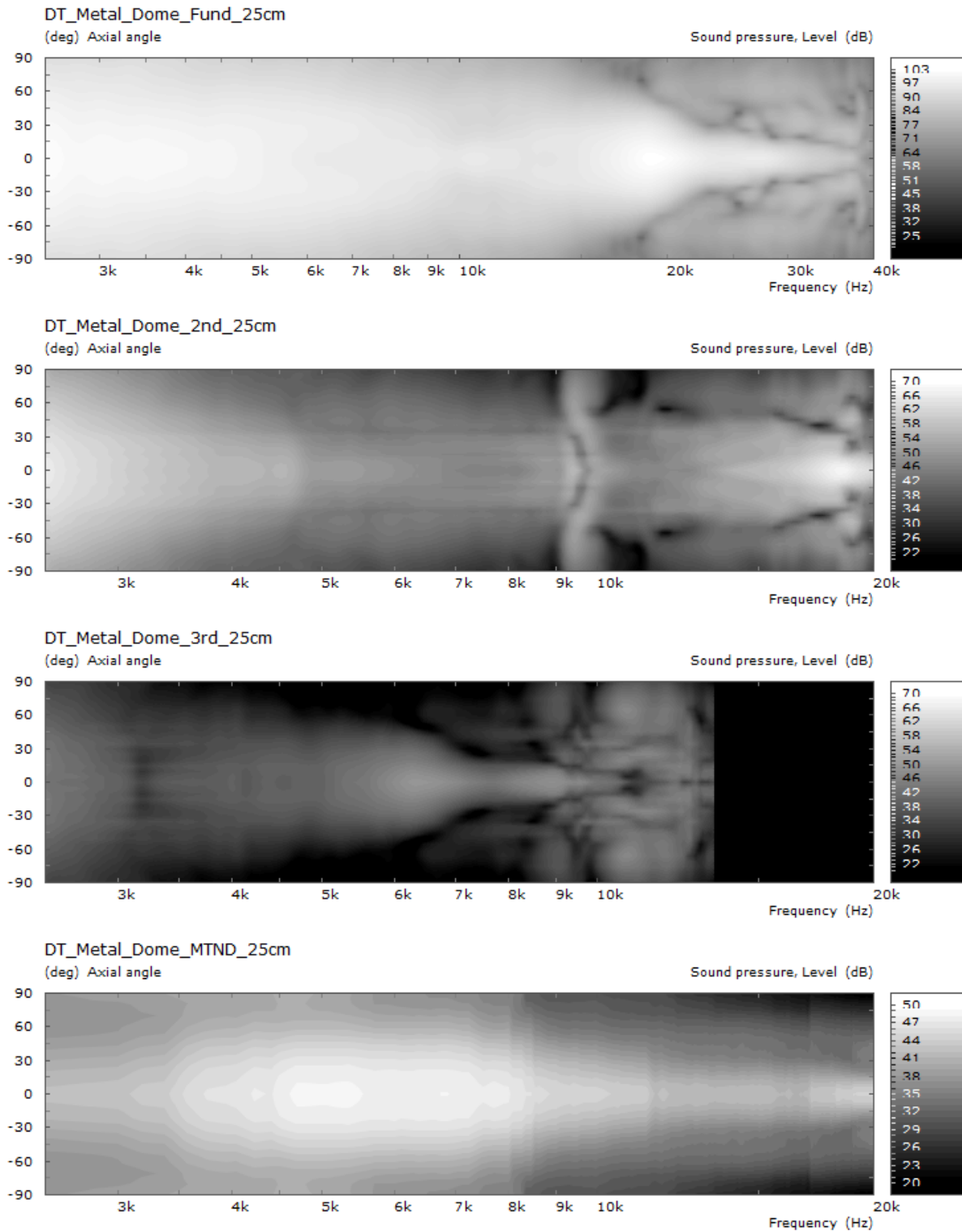
Figure 5: 25mm Metal Dome Tweeter
