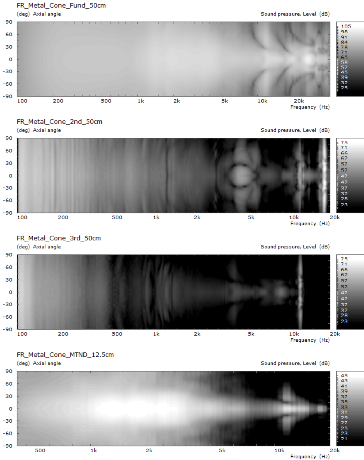
Figure 3: 76mm Full Range Metal Cone
