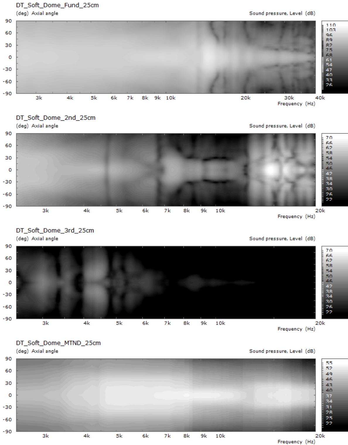
Figure 4: 25mm Soft Dome Tweeter
