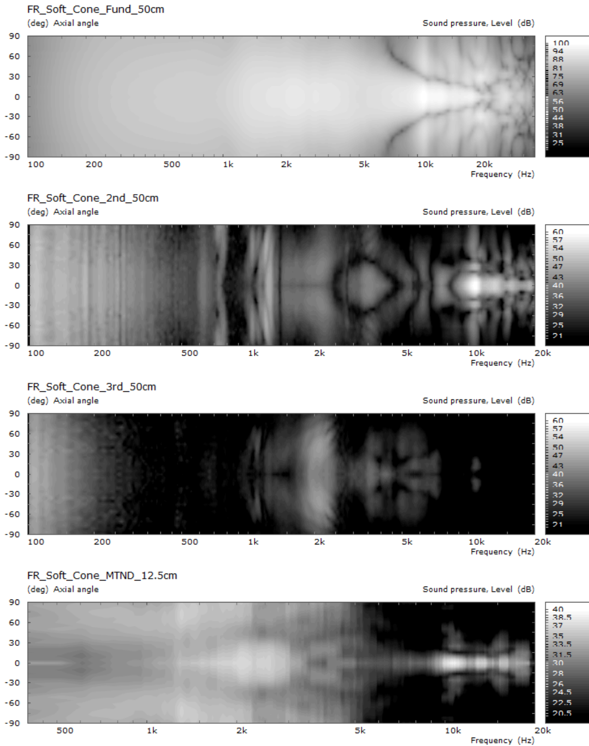
Figure 2: 76mm Full Range Soft Cone
