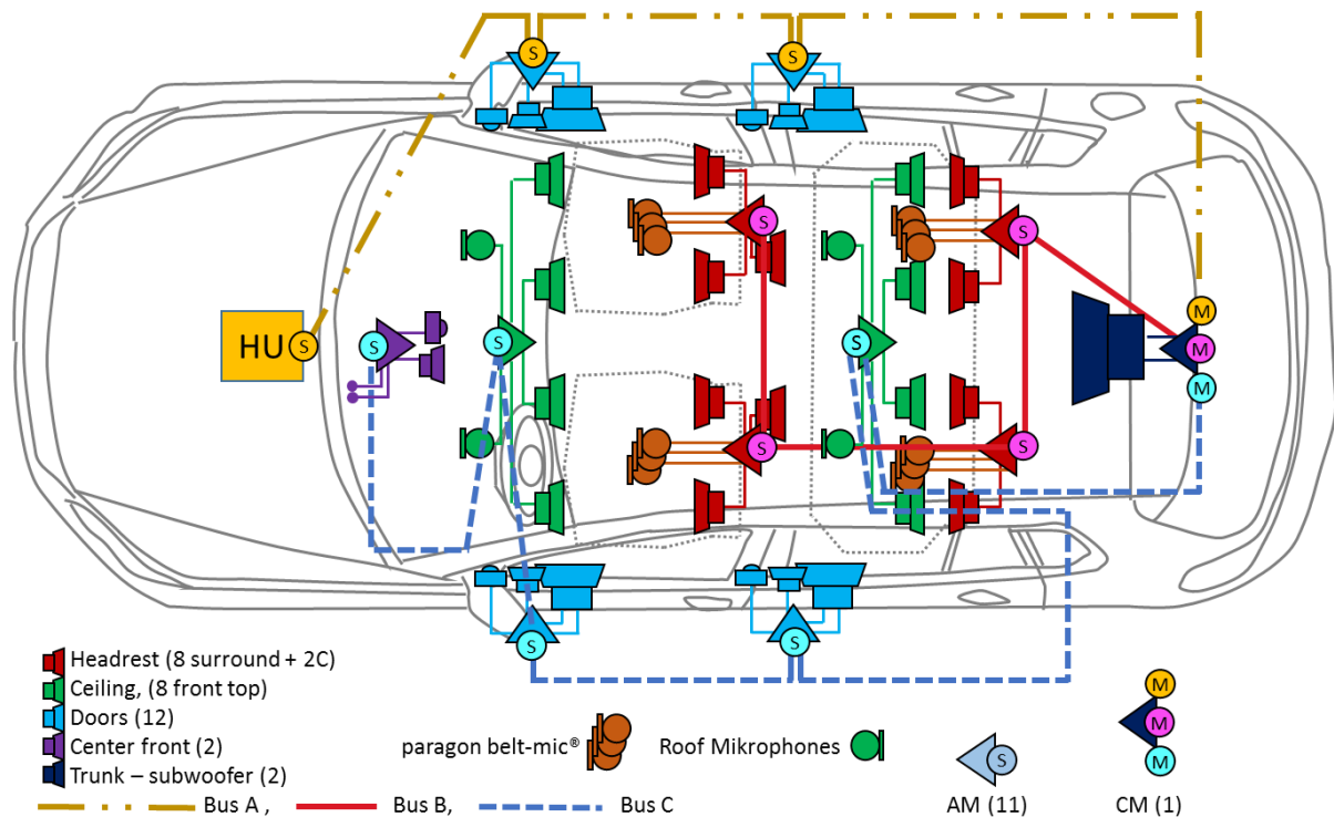
Figure 4. The demo car is equipped with a distributed system linked by 3 busses (A, B, C). The HU serves as a HMI, media source and telecommunication link. Entertainment and ICC processing is executed in a CM node. AM nodes close to loudspeakers carry out the loudspeaker management and mixing of speech signals. Class-D amplifiers drive 34 loudspeakers. 16 microphones are available for ICC and hands free telecommunication.
