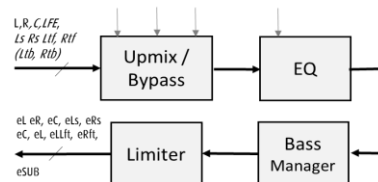
Figure 2. Entertainment processing blocks.
