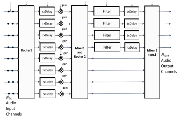
Figure 3. Programmable processing model of the loudspeaker management and signal mixing stages
