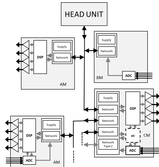
Figure 1. Distributed system with multiple busses and adapted nodes. The head unit (HU) is connected to a Computing Module (CM), which includes a multicore DSP and controller. It receives audio from the HU and the ADCs, executes the main processing tasks like entertainment and ICC and deploys the processed audio streams.
