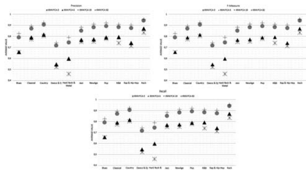
Fig. 4. Precision, Recall, and F-Measure metrics values for the k-NN algorithm.
