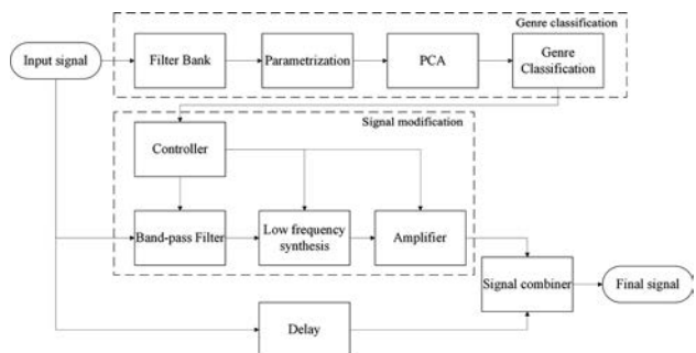
Fig. 6. Block diagram of proposed low frequency enhancement algorithm in a mobile device (Smart Virtual Bass Algorithm).
